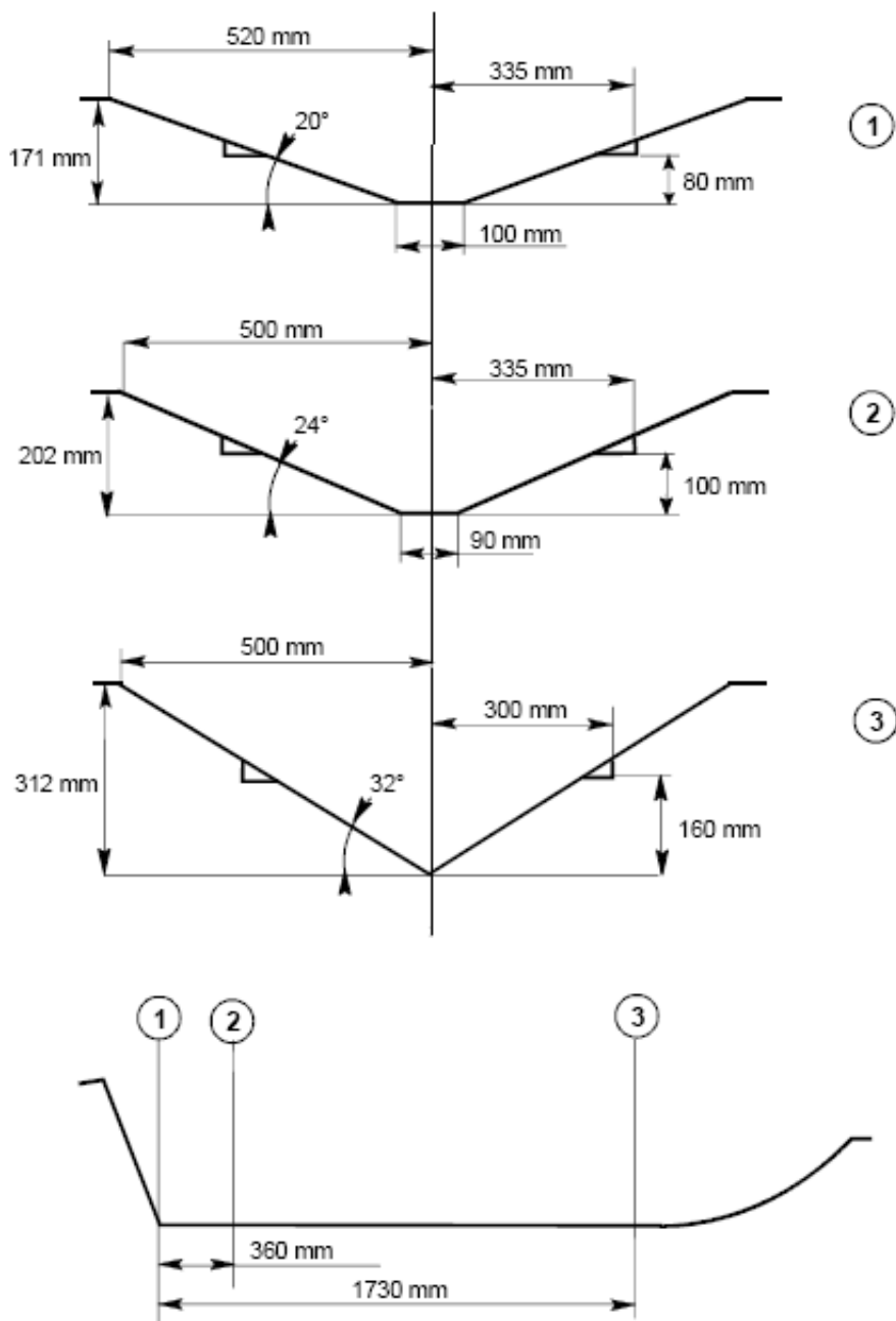
Hull profile
